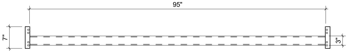
1 FRONT 3/4" = 1'-0"
